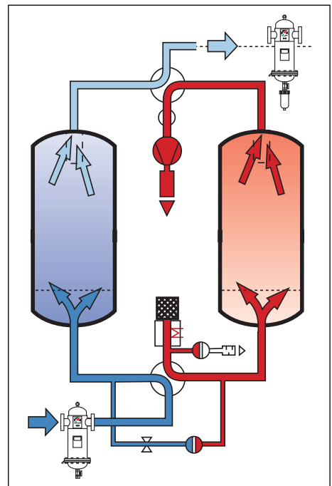
TZV schematic (recommended installation)
