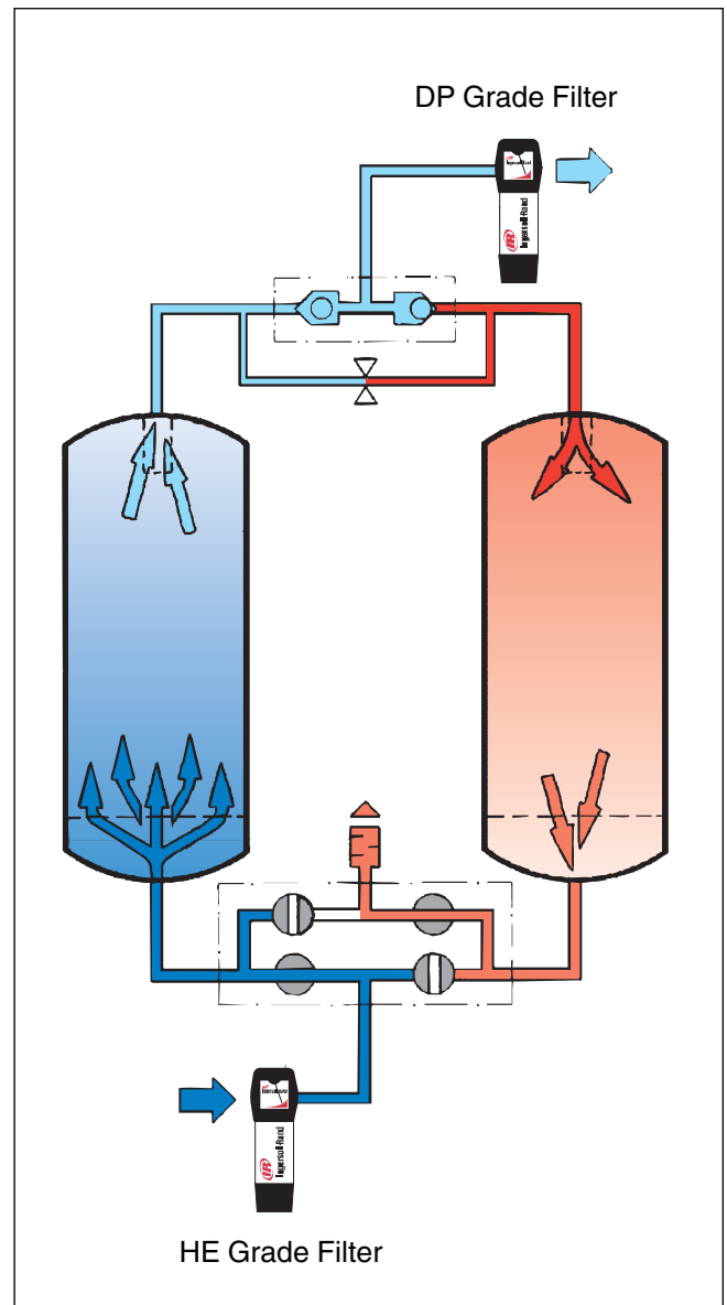
TZ 022-142 schematic (recommended installation)
